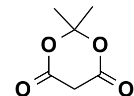
Meldrum's acid
